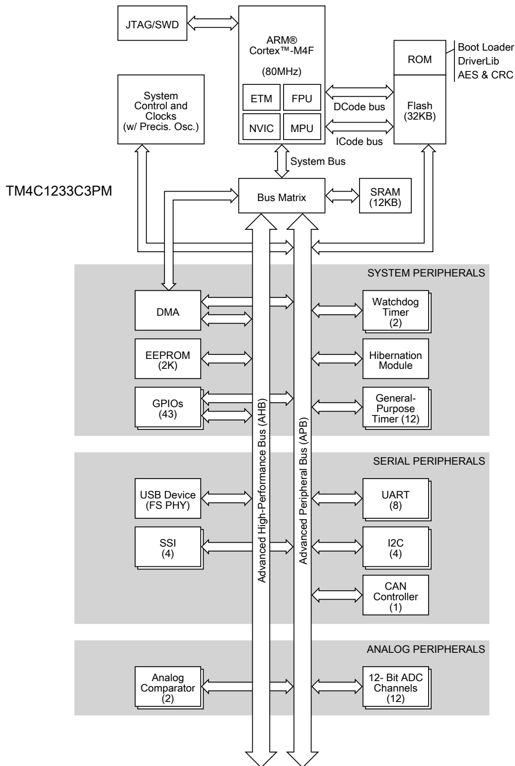
Figure 1-2. Tiva TM4C1233C3PM Microcontroller High-Level Block Diagram
